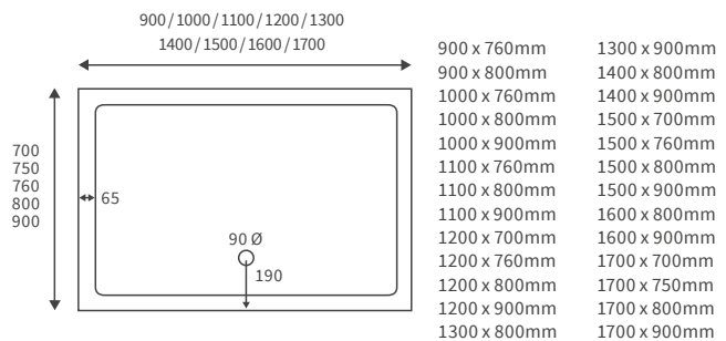
LOW PROFILE RECTANGULAR TRAYS
