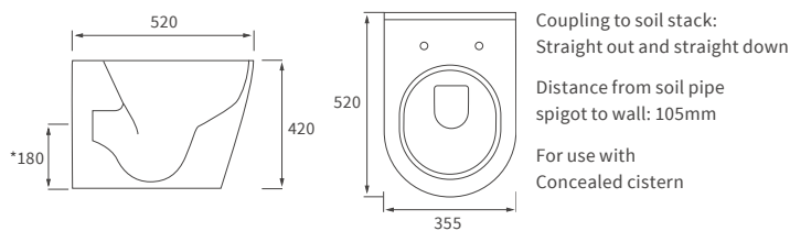
RIMLESS BACK TO WALL PAN
