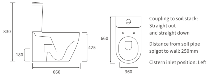
CLOSE COUPLED PAN AND CISTERN
