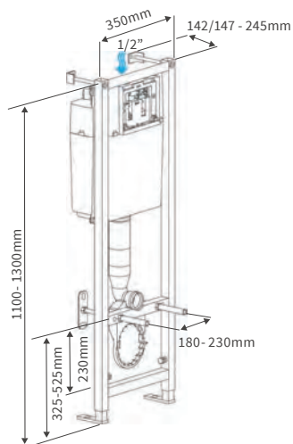
WALL HUNG WC FRAME
