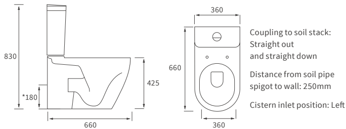
RIMLESS CLOSE COUPLED PAN AND CISTERN
