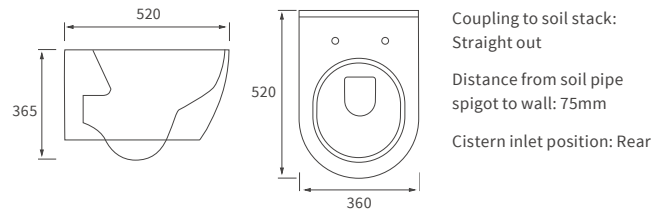
RIMLESS WALL HUNG PAN
